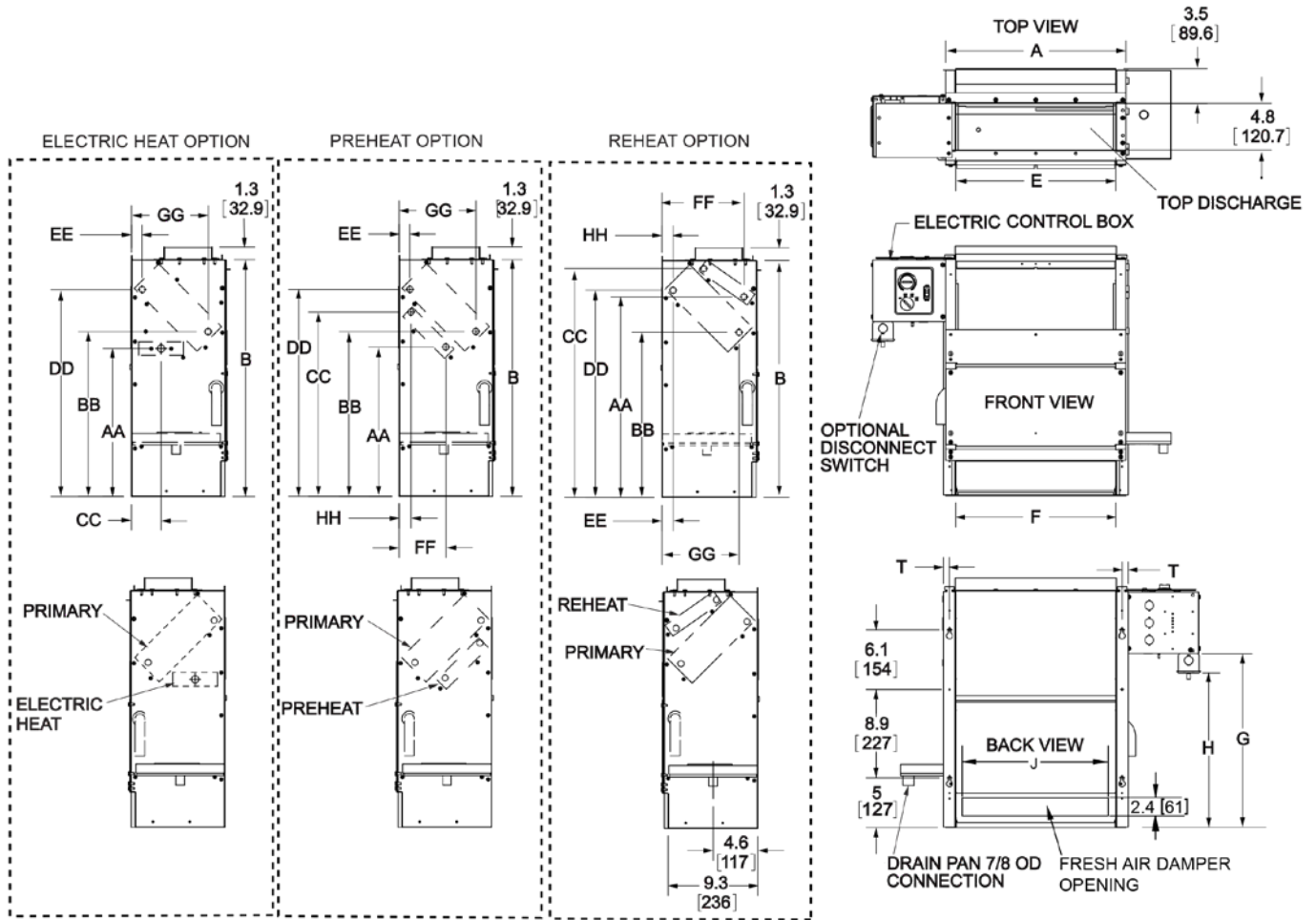
Figure 15: Dimensions: Hideaway, Top-Discharge Fan Coils
