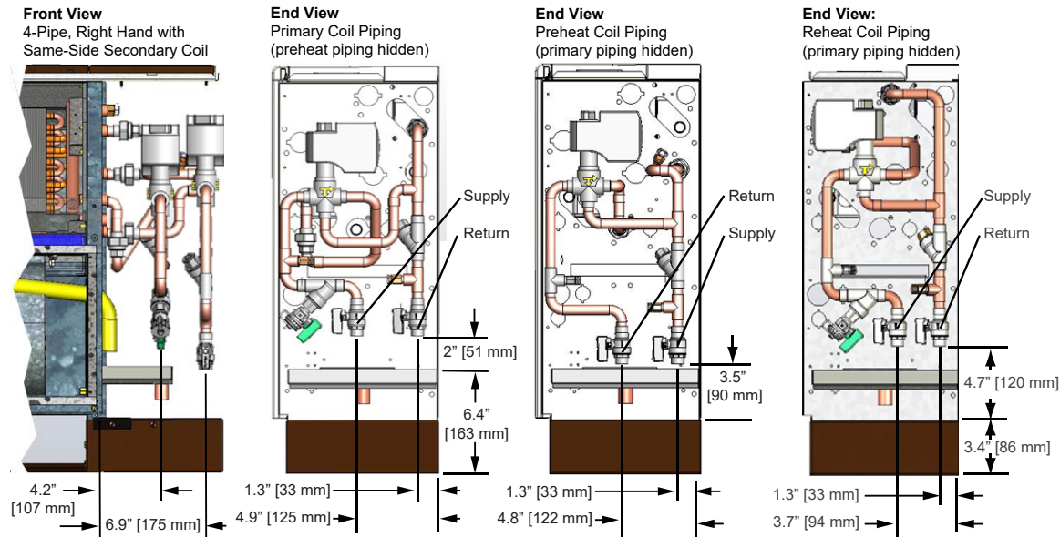
Figure 11: Hook Up Locations: Factory-Installed Valve and Piping Packages
