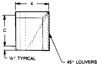
Figure 17: Fresh Air Intake Box Dimensions
