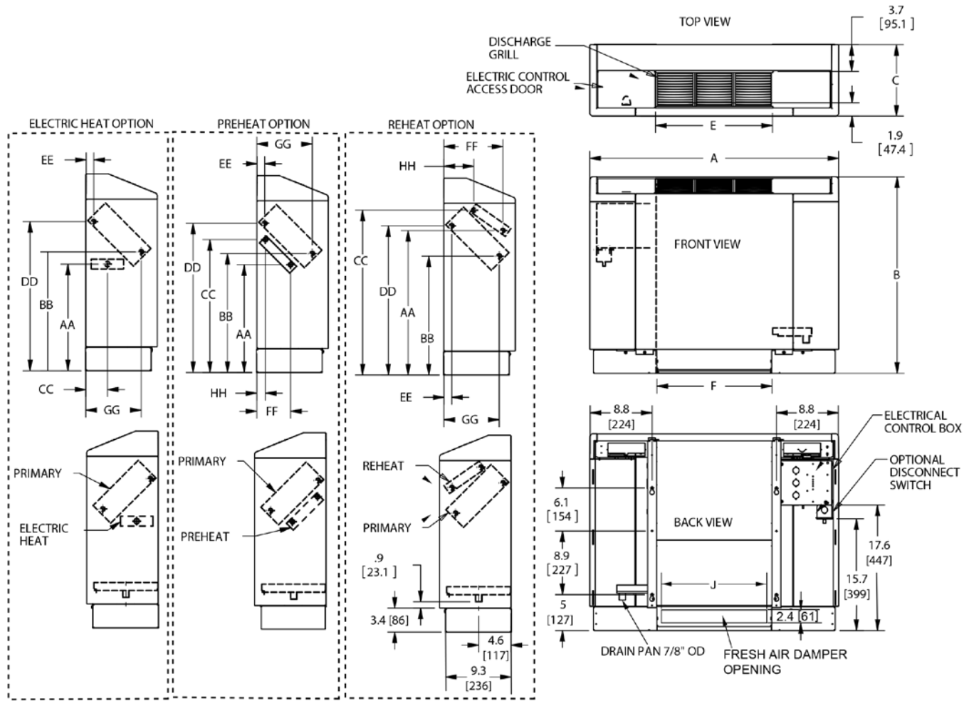
Figure 13: Dimensions: Slope Top Fan Coils
