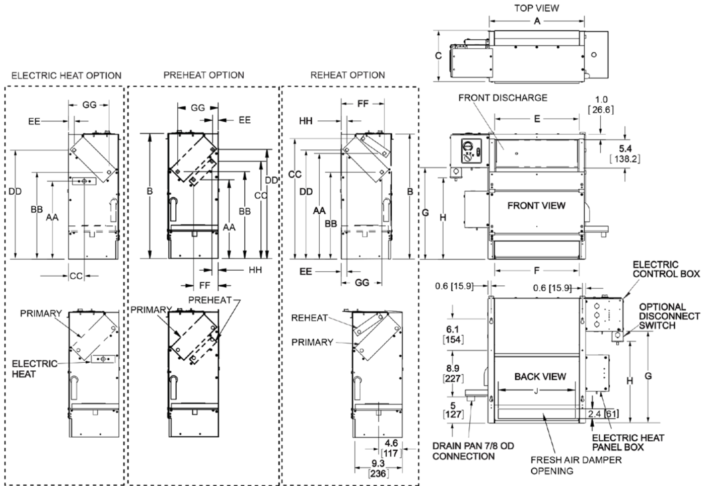
Figure 14: Dimensions: Hideaway, Front-Discharge Fan Coils
